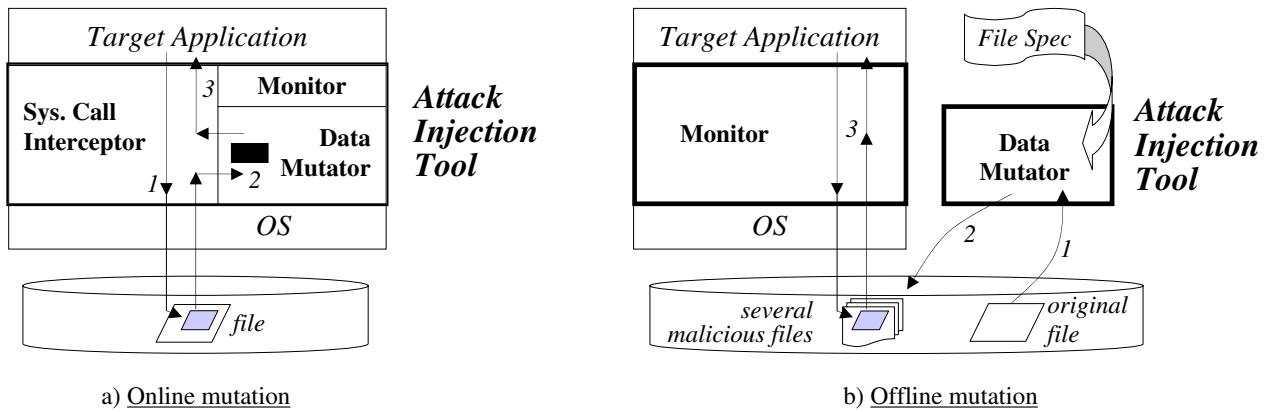
Figure 1. Attack injector with online and offline malicious file mutation.
